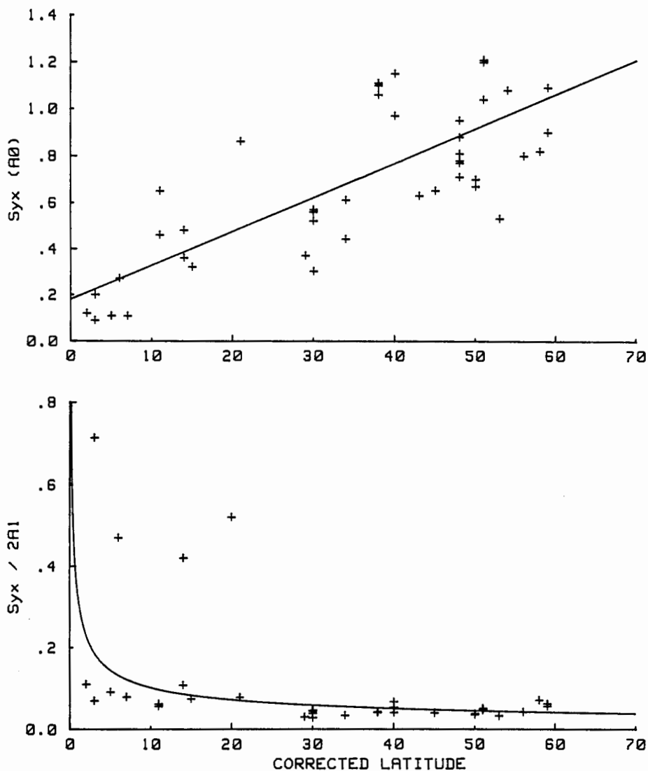
Fig. 6. The relative stochastic variability of water temperatures expressed as the ratio of the standard error of the estimate of the given parameters of periodic regression and the corresponding variable for average temperature and the annual amplitude ( A_0 and 2A_1 , respectively) plotted against corrected latitude. Upper panel - plot for the average temperature, lower panel - plot for the annual amplitude.
